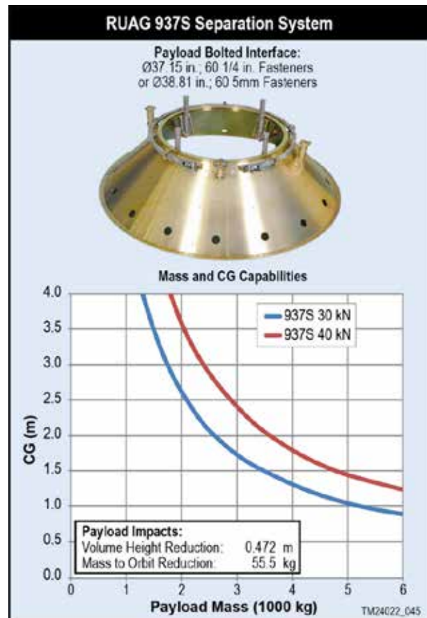
Figure 8.1.1-1. 937S Separation System
