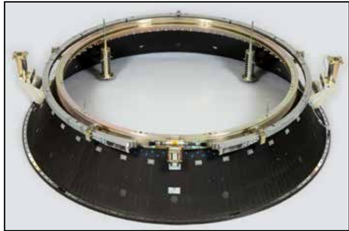
Figure 5.2.1-1. RUAG 1194 VS Payload Adapter
