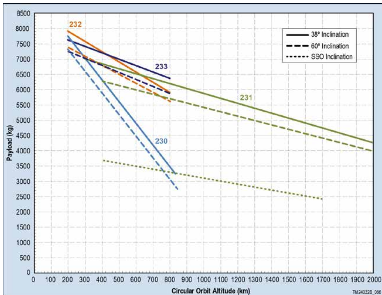
Figure 3.3-1. Antares Launch Capabilities from WFF
