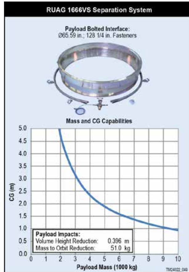
Figure 8.1.2-1. 1666VS Separation System
