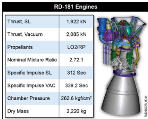
Figure 2.2.1-1. Antares Main Engine System
